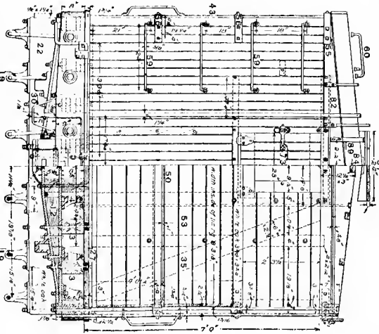
Fig. 253. Half End Elevation and Half Cross Section.
